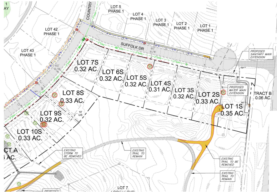
TREE REMOVAL PLAN
