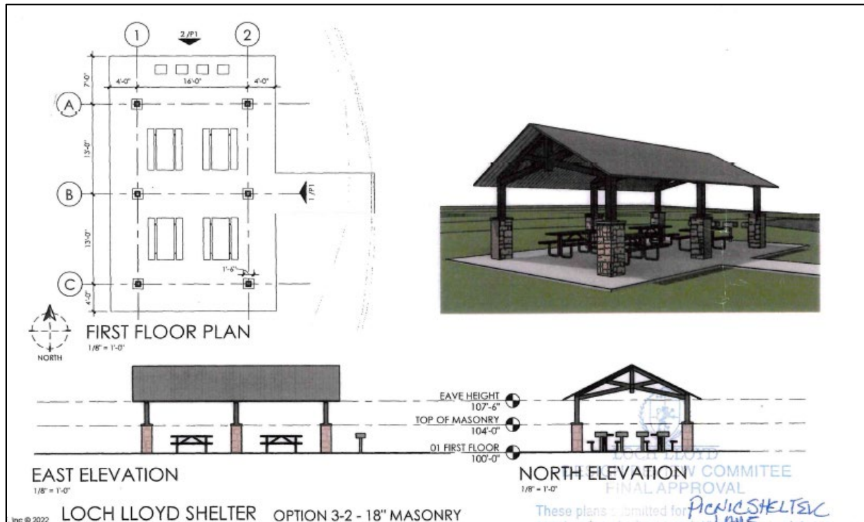
Building Elevations
